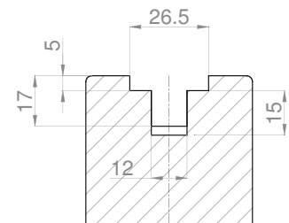
Section G-G
