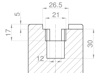
Section F-F
