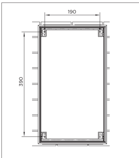
TAP wiring box: drilling template
